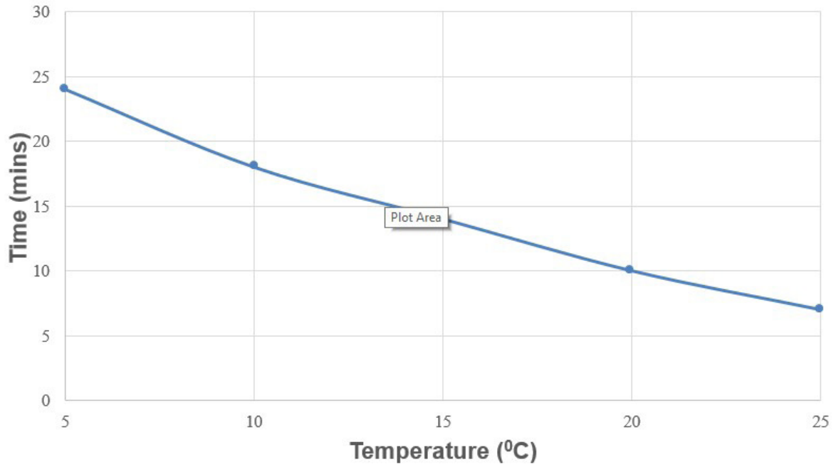
Time to achieve Barcol hardness of 75° versus temperature
